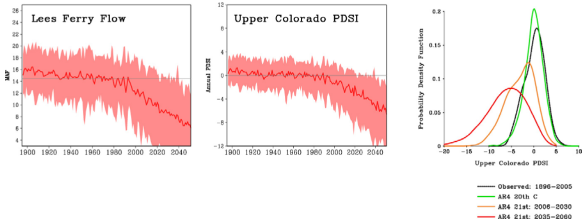
Plate B. The 1895-2050 Lees Ferry annual streamflow (left, maf) derived from the AR4 simulations of PDSI (middle) using the downscaling formula that relates observed Lees Ferry flow to observed PDSI during the 20 th century. The dark red curve denotes the 42-run average, and the cloud describes the 10 to 90 percent range of individual simulations. The right panel summarizes the probability distribution function of PDSI averaged over the Upper Colorado Drainage Basin for individual years of observations 1895-2005 (black), for the 42-models for 1895-2005 (green), and for the 42-model projections of the average PDSI during 2006-2030 (orange) and 2035-2060 (red). Note that the models produce a realistic range of PDSI drought events during the 20th century, and for the future they produce surface moisture conditions that denote progressive aridification and severe drought conditions.
