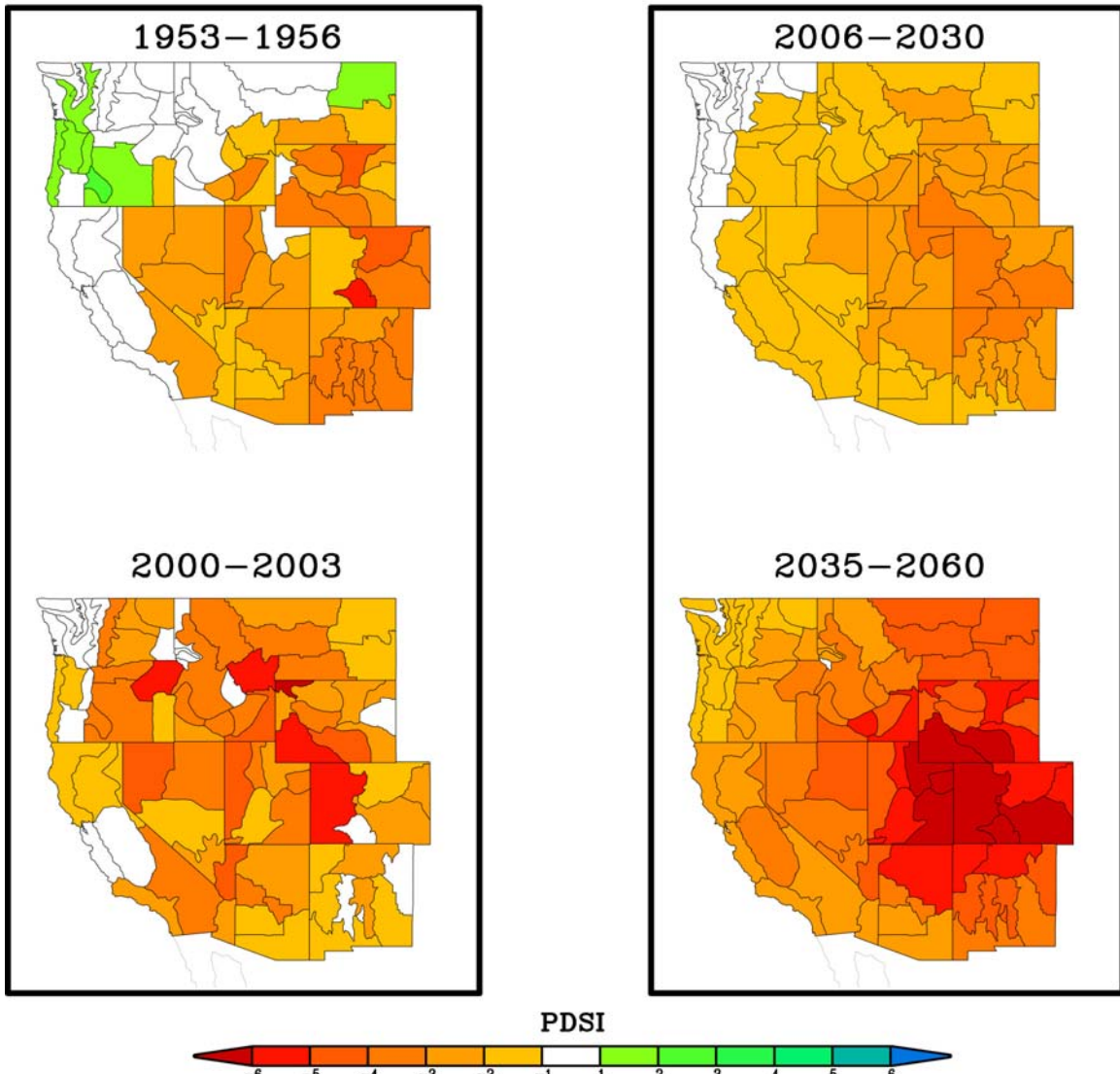
Plate A. Palmer Drought Severity Index (PDSI). Values less than -3 denote severe drought conditions. Left panels illustrate the 4-year average drought conditions experienced during the 1950s drought, and the recent drought. Right panels are future projections of the PDSI based on 42 simulations conducted to support the Fourth Assessment Report of the IPCC. By about 2050, average moisture balance conditions will mimic conditions experienced only rarely at the height of the most severe historical droughts.
